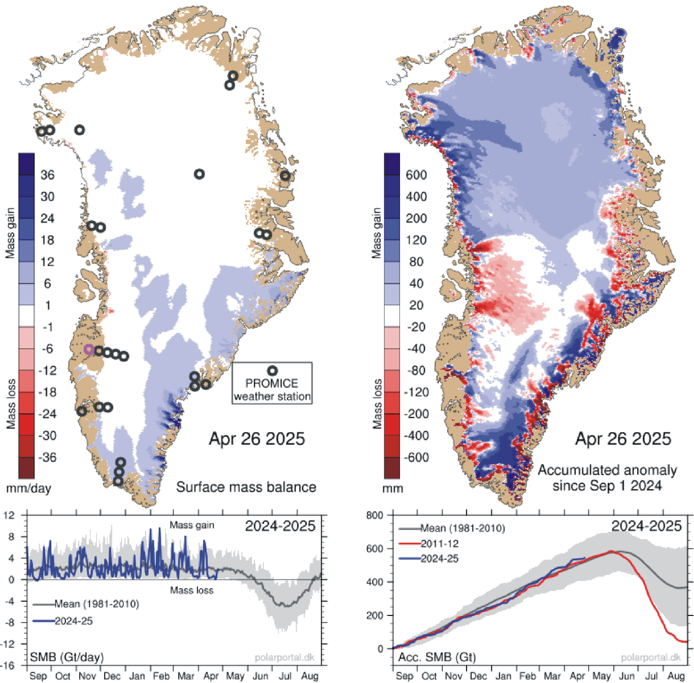
Left: Surface mass balance 26 April 2025. Right: Net surface mass balance anomaly since September 1, 2024. Courtesy of Danish Meteorological Institute (DMI).
