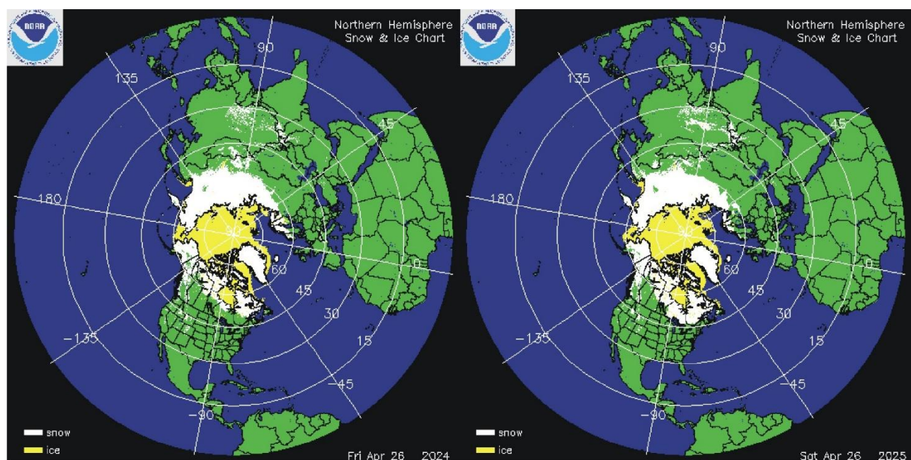
Northern hemisphere snow cover (white) and sea ice (yellow) 26 April 2024 (left) and 2025 (right). Map source: National Ice Center (NIC) .
