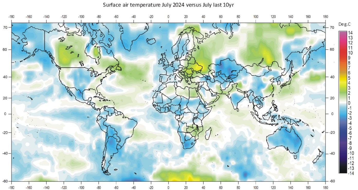
Surface air temperature July 2024 versus July last 10 yr
