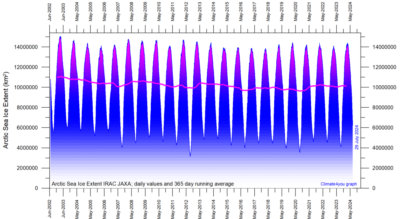
Diagram showing daily Arctic sea ice extent since June 2002, to 29 July 2024, data courtesy of Japan Aerospace Exploration Agency (JAXA) .
