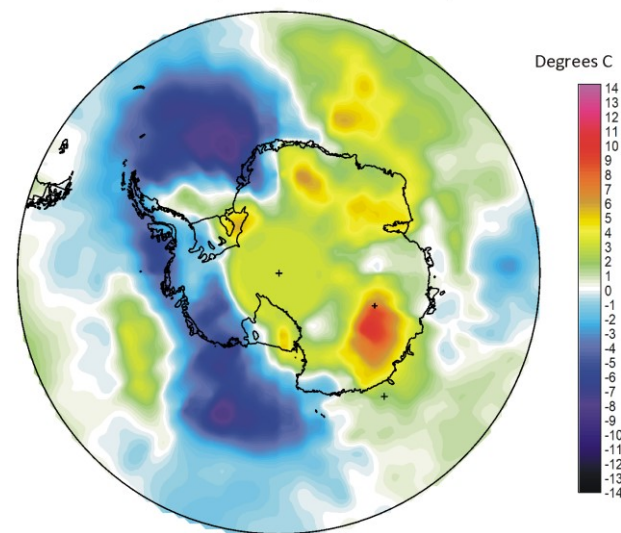
Surface air temperature July 2024 versus July 2023
