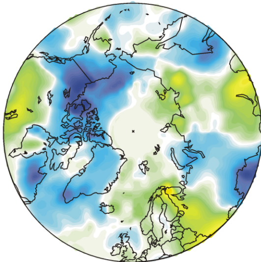
Surface air temperature July 2024 versus July 2023
