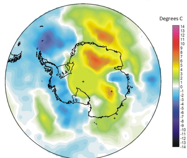
Surface air temperature July 2024 versus July last 10 yr
