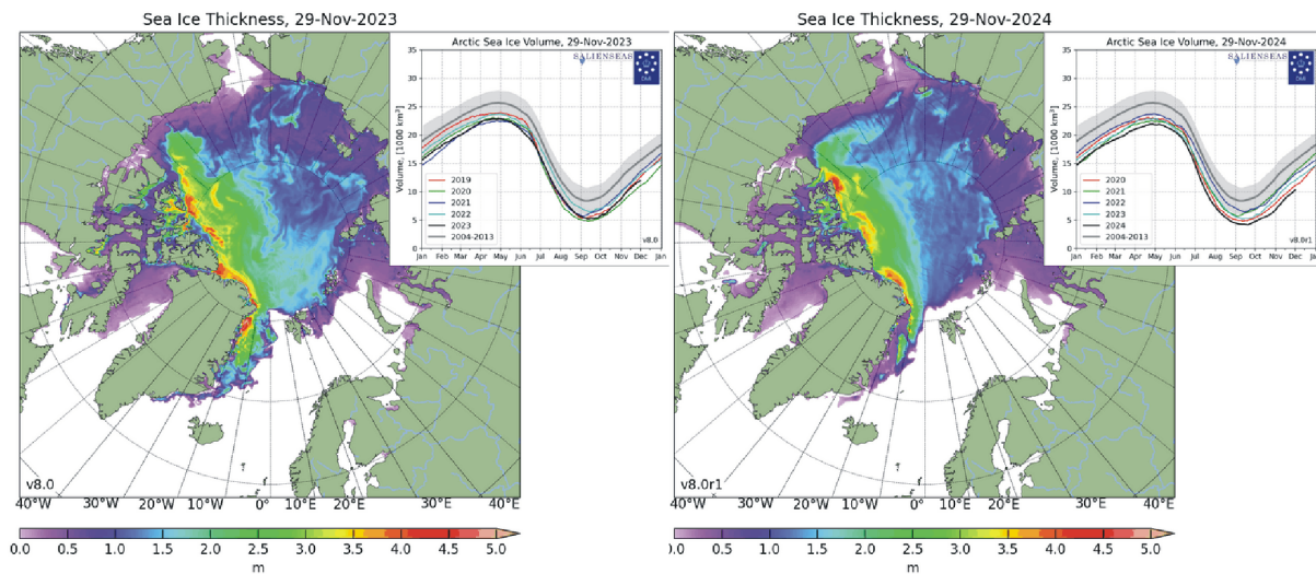
Diagrams showing Arctic sea ice extent and thickness 29 November 2023 (left) and 2024 (right and above) and the seasonal cycles of the calculated total arctic sea ice volume, according to The Danish Meteorological Institute (DMI) . The mean sea ice volume and standard deviation for the period 2004-2013 are shown by grey shading. Please note that DMI on 7 December 2021 changed their sea ice calculation model. DMI's description of the model version change can be read here: http://polarportal.dk/en/sea-ice-and-icebergs/sea-ice-thickness-and-volume/
