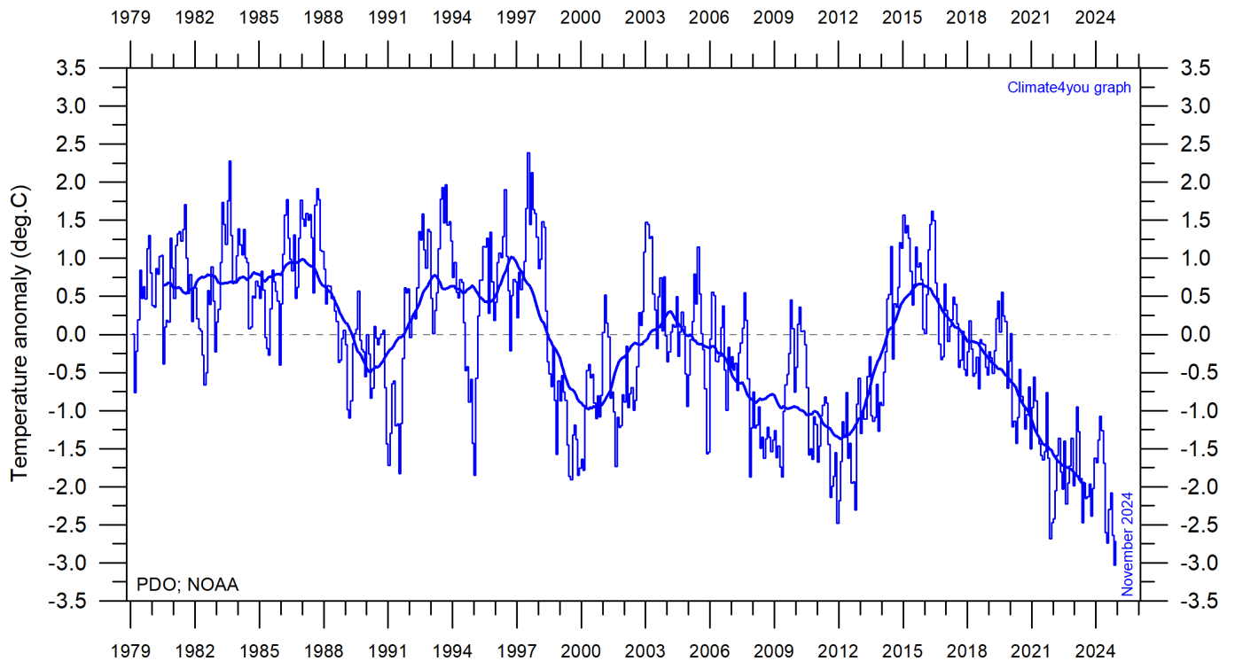
Monthly values of the Pacific Decadal Oscillation (PDO) since January 1979. The PDO is a long-lived El Niño-like pattern of Pacific climate variability, and the data series goes back to January 1854. Base period: 1982-2002. The thin line indicates monthly PDO values, and the thick line is the simple running 37-month average. Data source: NOAA Physical Science Laboratory (version PDO ERSST V5 plotted above).
