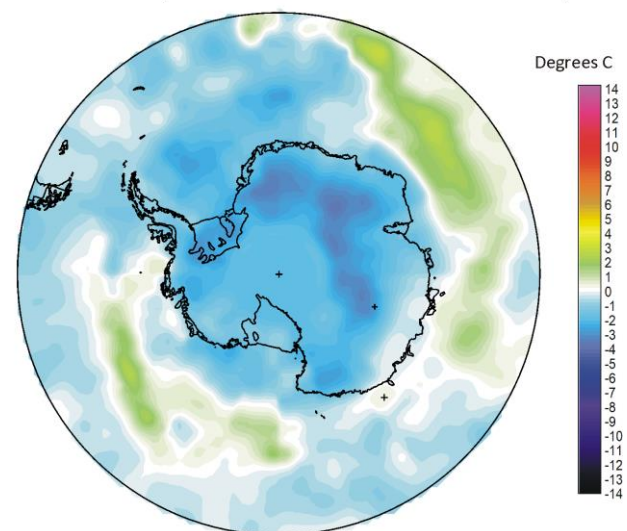
Surface air temperature November 2024 versus November last 10 yr
