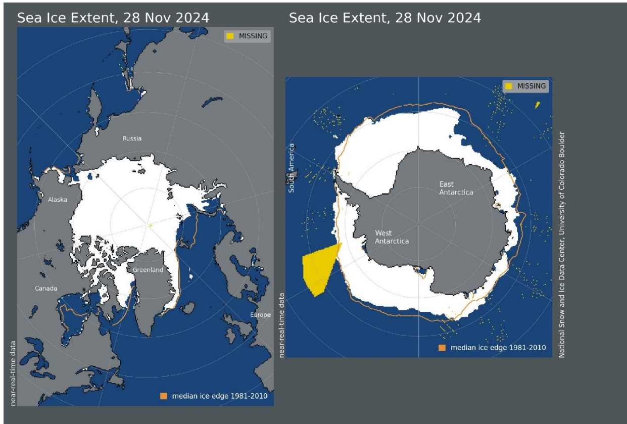
Sea ice extent 28 November 2024. The median limit of sea ice (orange line) is defined as 15% sea ice cover, according to the average of satellite observations 1981-2010 (both years included). Sea ice may therefore well be encountered outside and open water areas inside the limit shown in the diagrams above. Map source: National Snow and Ice Data Center (NSIDC).
