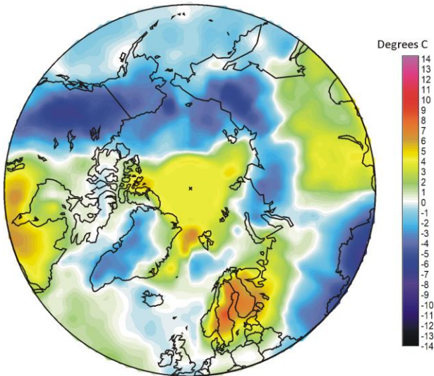
Surface air temperature November 2024 versus November 2023
