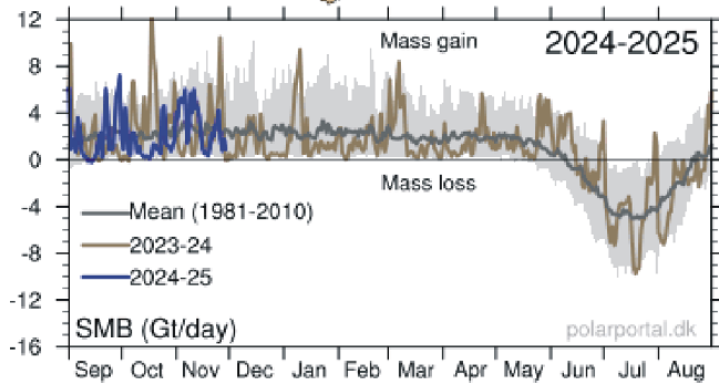
Left: Surface mass balance 29 November 2024. Right: Net surface mass balance anomaly since September 1, 2024. Courtesy of Danish Meteorological Institute (DMI).
