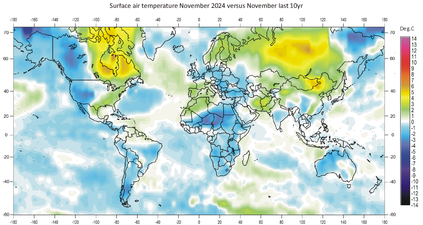
Surface air temperature November 2024 versus November last 10 yr
