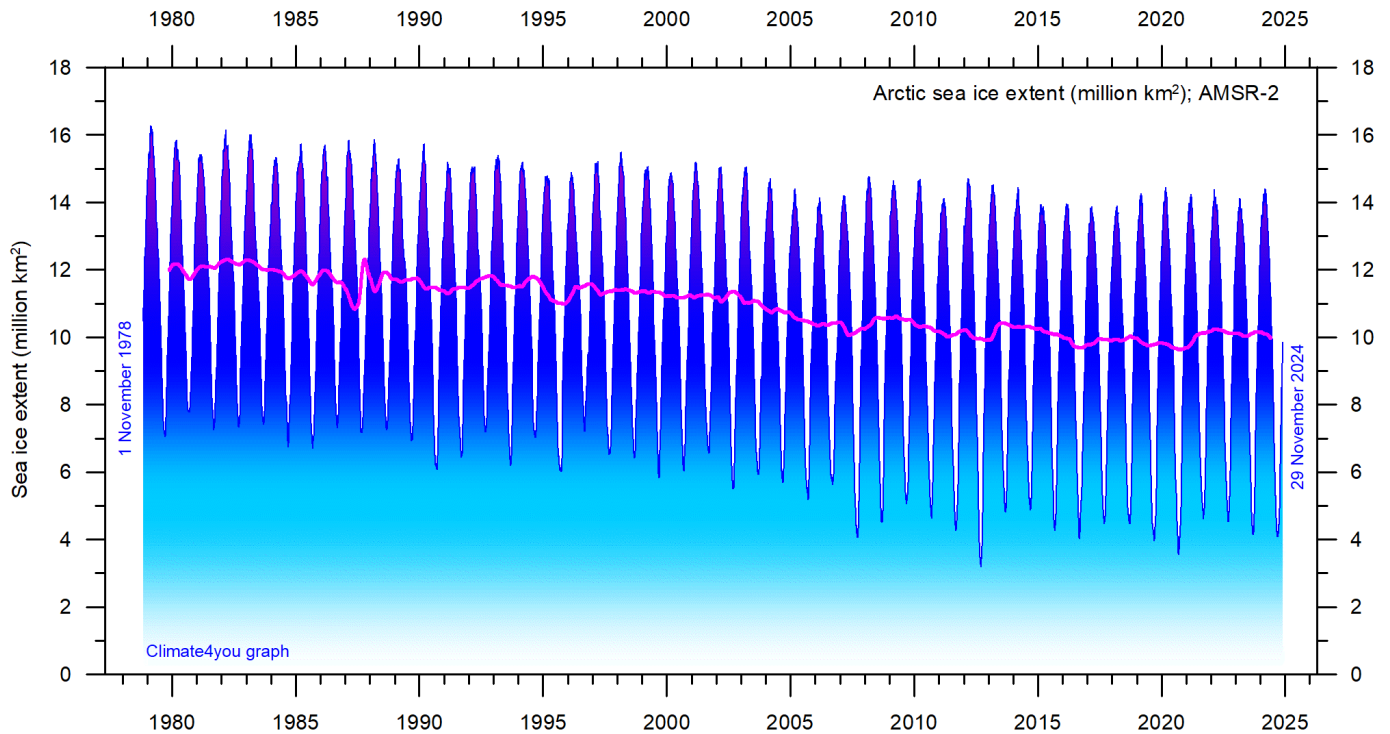
Diagram showing daily Arctic sea ice extent since November 1978, to 29 November 2024, data courtesy of Japan Aerospace Exploration Agency (JAXA) .
